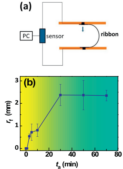
Fig. 4. (a) Schematic illustration of the apparatus for bending plasticity test. The displacement rate is 1 mm/min. The fracture radius ( r_f ) is detected automatically. (b) The evolution of fracture radius along with annealing time t_a .
