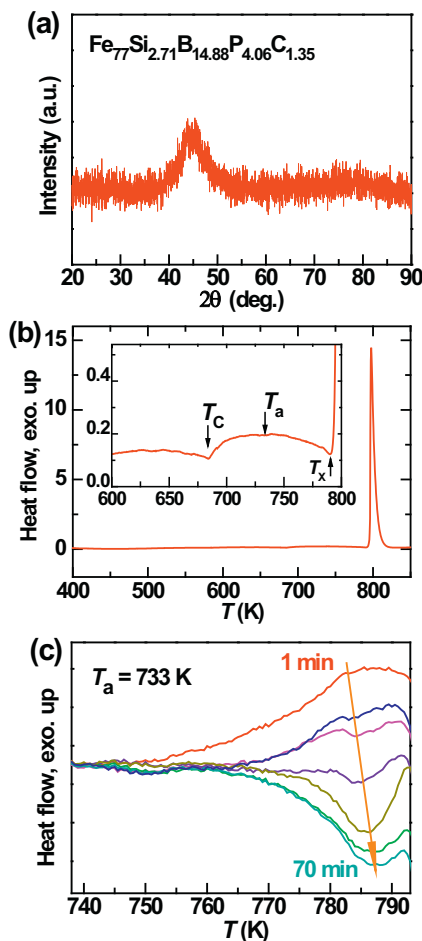
Fig. 1. (a) The XRD pattern of the as-spun Fe 77 Si 2.71 B 14.88 P 4.06 C 1.35 ribbon. (b) The DSC trace of Fe 77 Si 2.71 B 14.88 P 4.06 C 1.35 metallic glass at heating rate of 40 K/min. The inset is the magnified part close to Curie temperature T_C and crystallization temperature T_x . (c) Change of heat flows after being annealed at 733 K for various times.
