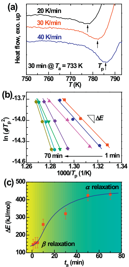
Fig. 2. (a) The heat flows at different heating rates for the sample preannealed at 733 K for 30 min. (b) The Kissinger plot of the relaxation peak for samples preannealed at 733 K for various time. (c) The evolution of relaxation barrier along with annealing time t_a . The yellow background zone represents \beta relaxation stage and the cyan background represents \alpha relaxation stage.
