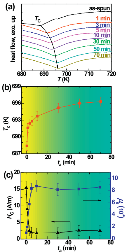
Fig. 3. (a) The DSC traces close to the magnetic phase transition range for samples preannealed at 733 K for various time, with a curve showing the change of T_C . (b) The evolution of T_C along with t_a . (c) The evolution of H_C (left axis) and \mu_e (right axis) along with annealing time t_a .
