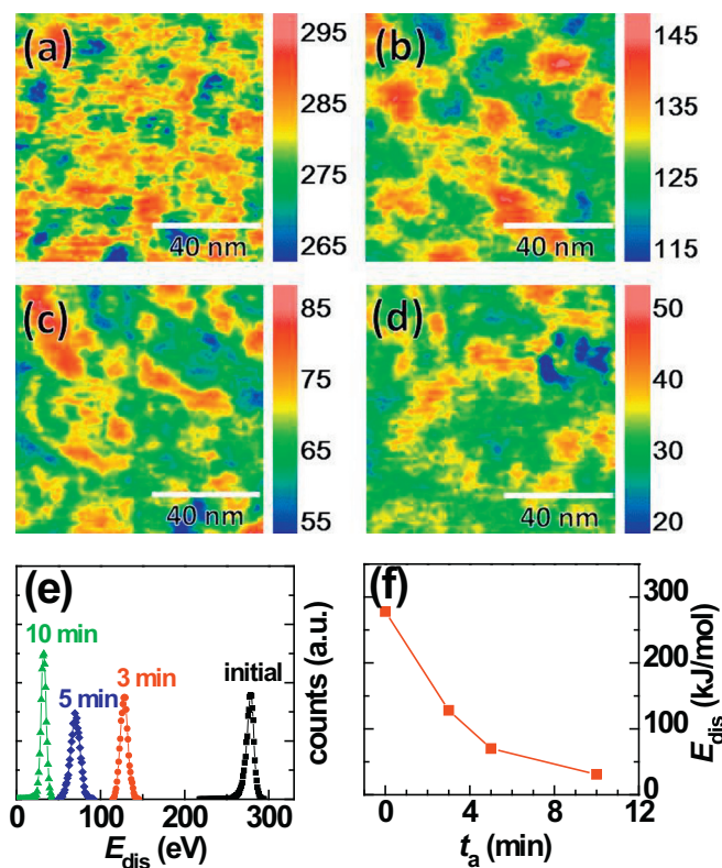
Fig. 5. The nanoscale viscoelastic heterogeneity for samples annealed at 733 K for different times (a) as-spun, (b) t_a = 3 min, (c) t_a = 5 min, (d) t_a = 10 min. The color bar represents E_{dis} , in unit of eV. (e) The statistical distribution of dissipation energy E_{dis} for as-spun and annealed samples. (f) The evolution of E_{dis} (peak value) along with annealing time t_a .
