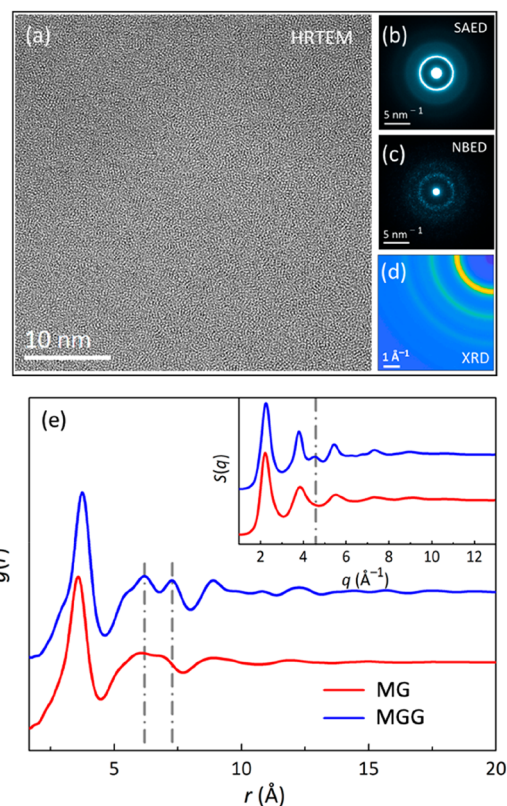
Figure 3. Structural characterization of the MGG. No crystalline phases are detected under the examination of high-resolution transmission electron microscopy (HRTEM) imaging (a), selected area electron diffraction (SAED) (b), nanobeam electron diffraction (NBED) (c), and synchrotron X-ray diffraction (SXR) (d). The pair correlation function g(r) and the structural factor S(q) (inset) of the MG and the MGG are compared in panel e. The split of the second peak in both g(r) and S(q) of the MGG is marked by dotted lines.
